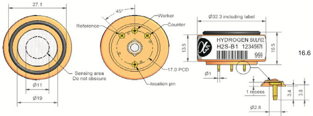
Figure 1 H2S-B1 Schematic Diagram
