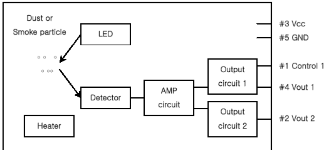
FIGURE 1.1. BLOCK DIAGRAM
