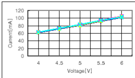
FIGURE 4.1. VOLTAGE VS CURRENT
